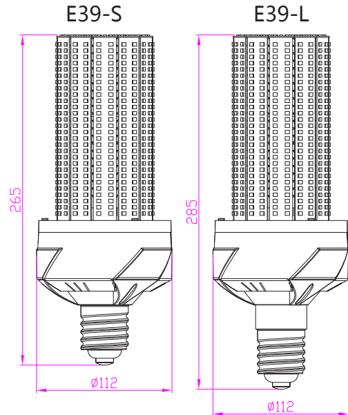
E39-S: Short Plastic Housing
