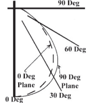
Photometric Curve
