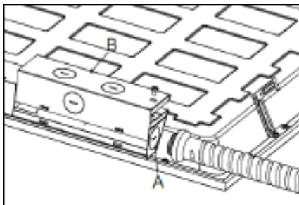
1. Remove the knock down hole on box by screwdriver.
