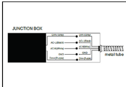
2. Connect the wire as the picture shows.
