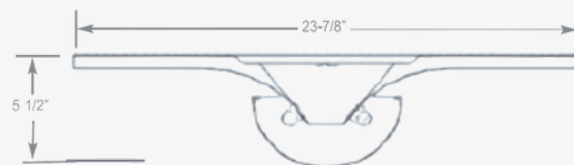
2x2/2x4-2-Lamp Perforated Basket
