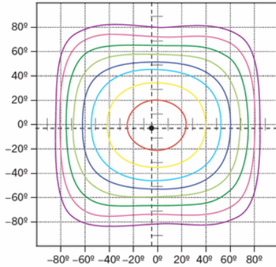
ISOCANDELA PLOT
