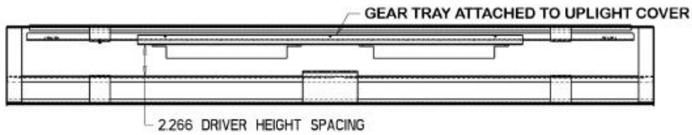
BOTTOM VIEW (DOWNLIGHT)
